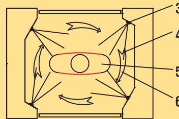
3. Fixed Nozzle 4. High Velocity Airflow 5. Body 6. Ring Airflow
