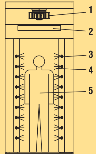
1. Blower 2. HEPA Filter 3. Fixed Nozzle 4. High Velocity Airflow 5. Body
